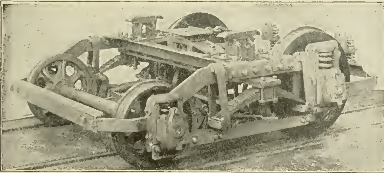
Fig. 15. Maximum Traction Truck
